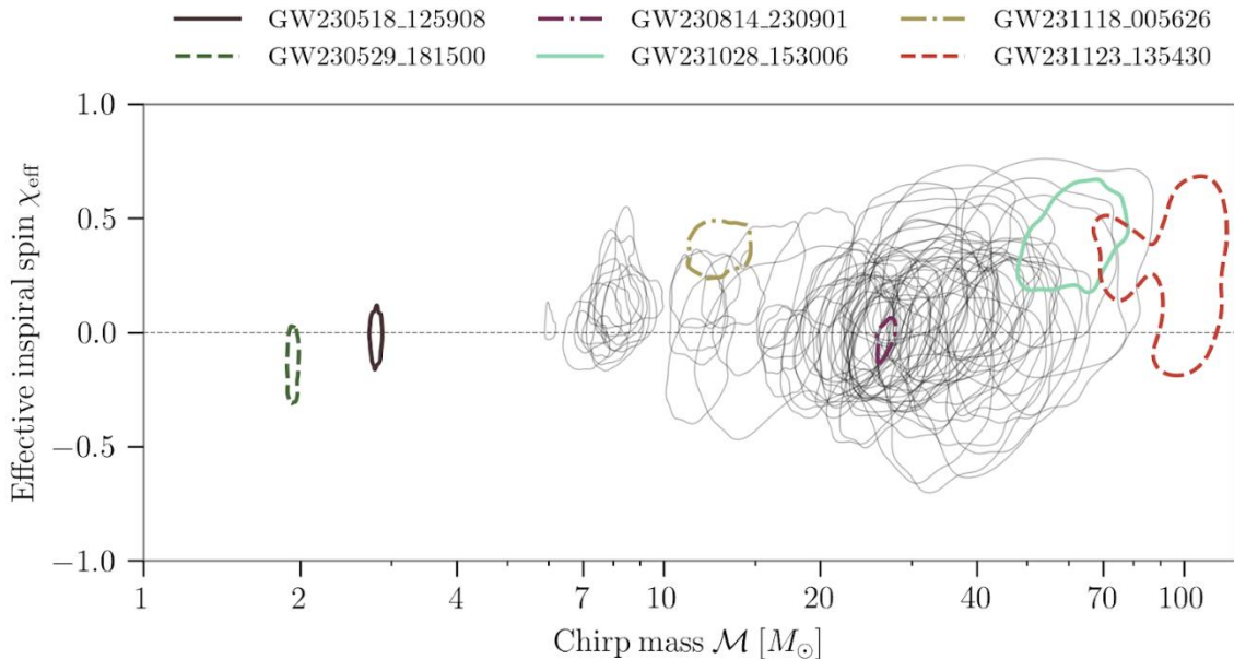
Figure 4: A plot of the chirp mass against the effective spin for all of the new candidates in GWTC-4.0 with a selection of especially interesting candidates highlighted in color. Each contour encloses the 90% confidence region for the parameters of that candidate.
