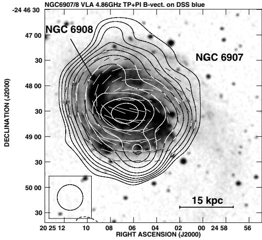
Fig. 7. The total power contours and \mathbf{B} -vectors of polarized intensity of NGC 6907/NGC 6908 at 4.86 GHz (natural weighting) superimposed on the DSS blue image. The contour levels are (-3, 3, 5, 8, 12, 20, 35, 80, 150, 250, 400) \times 32.0 \mu\text{Jy}/\text{beam} . A vector of 10'' length corresponds to the polarized intensity of 125.0 \mu\text{Jy}/\text{beam} . The map resolution is 30'' \times 30'' HPBW.
