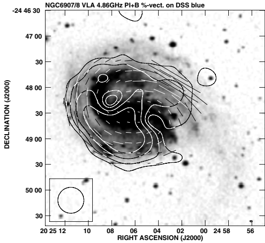
Fig. 8. The contours of polarized intensity and \mathbf{B} -vectors of polarization degree of NGC 6907/NGC 6908 at 4.86 GHz (natural weighting) superimposed on the DSS blue image. The contour levels are (3, 5, 8, 12) \times 23.3 \mu\text{Jy}/\text{beam} . A vector of 10'' length corresponds to the polarization degree of 8%. The map resolution is 30'' \times 30'' HPBW.
