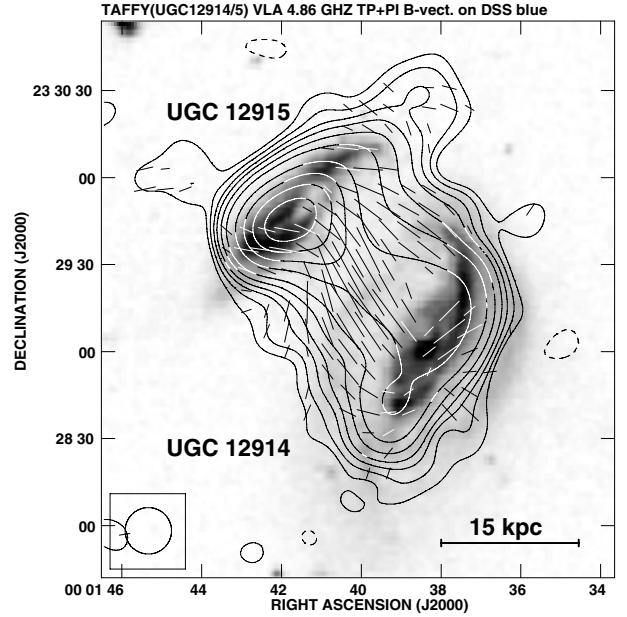
Fig. 9. The total power contours and \mathbf{B} -vectors of polarized intensity of the Taffy (UGC 12914/UGC 12915) at 4.86 GHz superimposed on the DSS blue image. The contour levels are (-3, 3, 5, 8, 12, 20, 35, 80, 150, 250, 400) \times 17.0 \mu\text{Jy}/\text{beam} . A vector of 10'' length corresponds to the polarized intensity of 71.4 \mu\text{Jy}/\text{beam} . The map resolution is 16'' \times 16'' HPBW.
