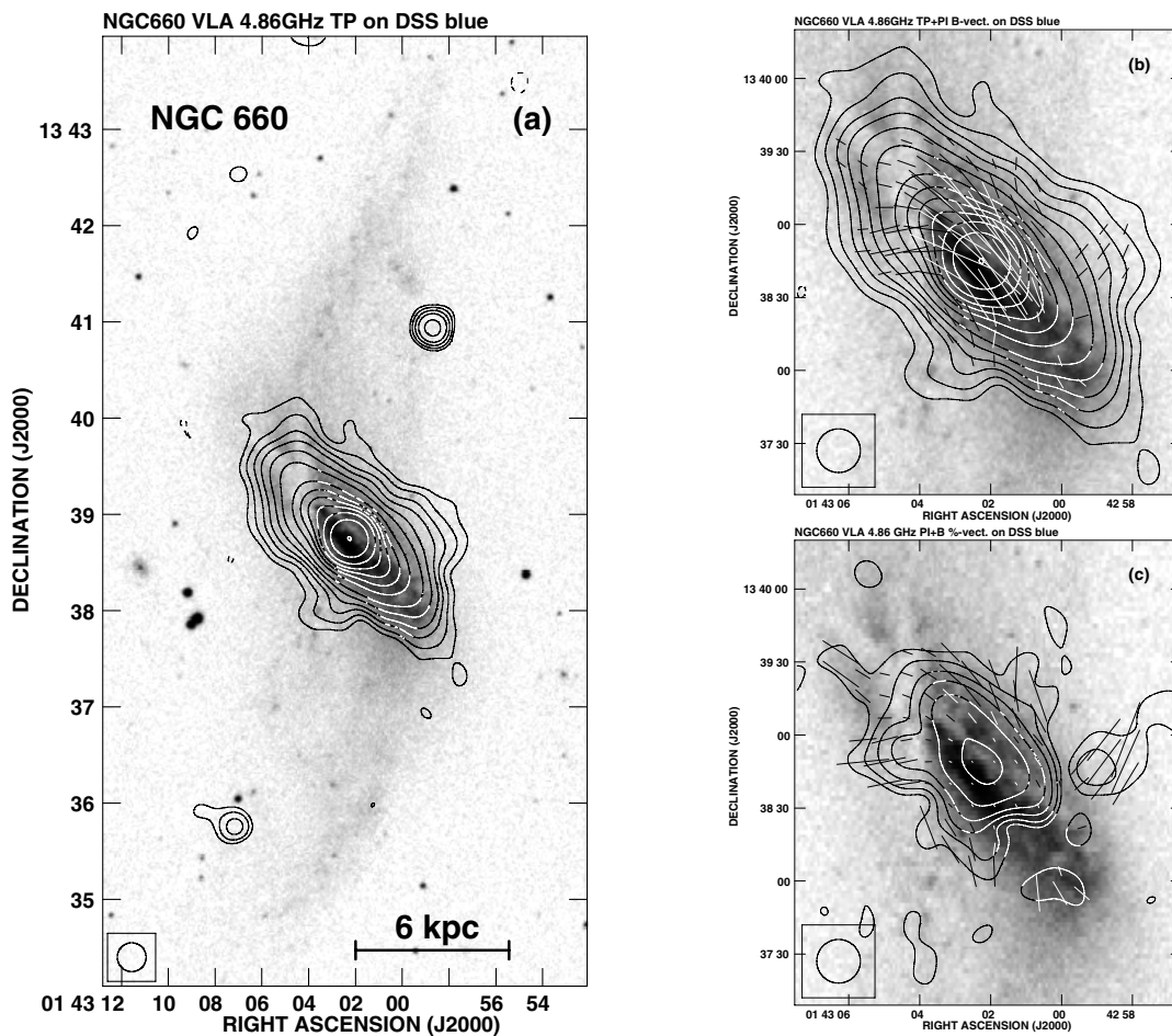
Fig. 11. a) The total power contours of NGC 660 at 4.86 GHz (natural weighting) superimposed on the DSS blue image. A large warped ring in the NS direction is visible. The contour levels are (-3, 3, 5, 8, 12, 20, 35, 80, 150, 250, 400, 700, 1500, 4000) \times 26.4 \mu\text{Jy}/\text{beam} . b) The total power contours and \mathbf{B} -vectors of polarized intensity of the disk of NGC 660 superimposed on DSS blue image. The contour levels are the same as for a) . A vector of 10'' length corresponds to the polarized intensity of 100.0 \mu\text{Jy}/\text{beam} . c) The contours of polarized intensity and \mathbf{B} -vectors of polarization degree of the disk of NGC 660 at 4.86 GHz (natural weighting) superimposed on the DSS blue image. The contour levels are (3, 5, 8, 12, 20, 35) \times 13.4 \mu\text{Jy}/\text{beam} . A vector of 10'' length corresponds to the polarization degree of 11%. The maps resolution is 18'' \times 18'' HPBW.
