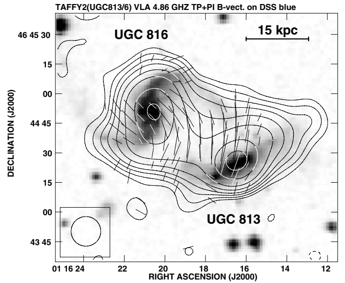
Fig. 10. The total power contours and \mathbf{B} -vectors of polarized intensity of the Taffy2 (UGC 813/UGC 816) at 4.86 GHz superimposed on the DSS blue image. The contour levels are (-3, 3, 5, 8, 12, 20, 35, 80, 150) \times 23.0 \mu\text{Jy}/\text{beam} . A vector of 10'' length corresponds to the polarized intensity of 69.4 \mu\text{Jy}/\text{beam} . The map resolution is 15'' \times 15'' HPBW.
