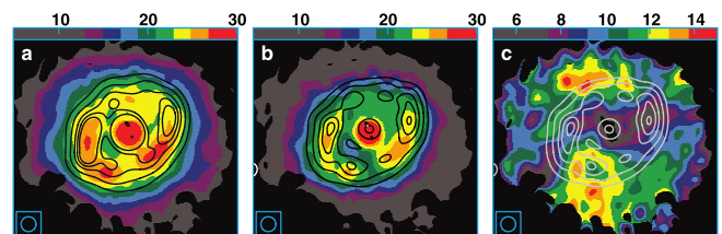
FIG. 5.—Magnetic maps of NGC 4736. (a) Total, (b) random, and (c) regular magnetic field strength (in \mu\text{G} ) in colors, with contours of (a) infrared 24 \mu\text{m} and (b, c) H \alpha emission.
